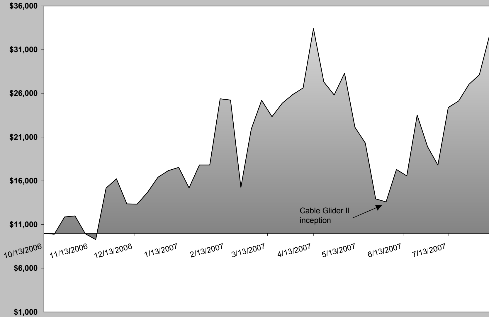
Cable Glider I and II (October 2006 - Present ) Model Risk Capital Returns
